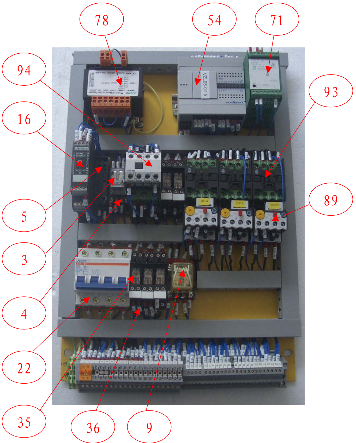
MC2 Pinsetter Control Box With Pit Light exchanging Control *Used in MC2
