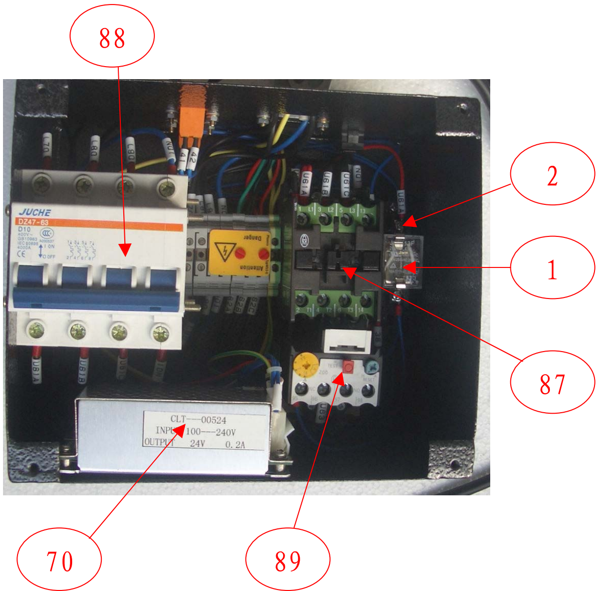
Power Lift Control Box
